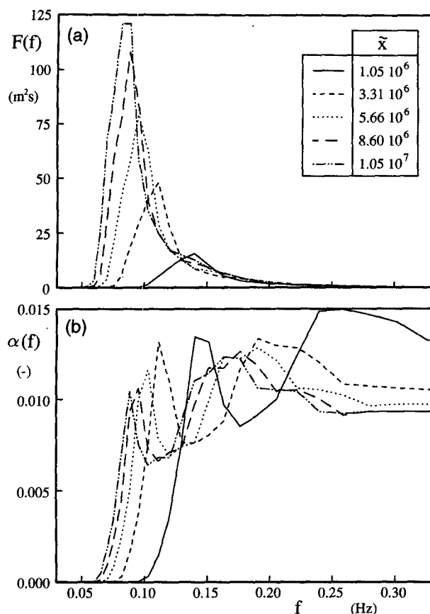
FIG. 8. One-dimensional energy spectra \mathcal{R}(f) (a) and nondimensional energy level \alpha(f) [Eq. (26)] (b) for several fetches \bar{x} corresponding to the growth curves of Fig. 7 (model tuned to stable stratification data, \Delta x = 25 km).
