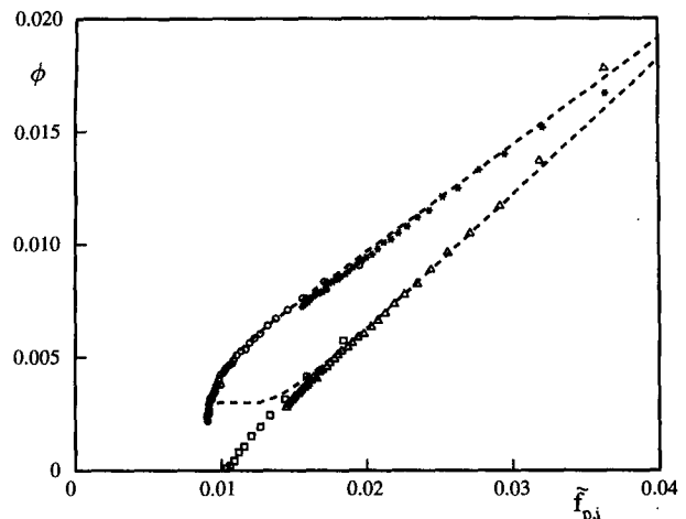
FIG. 6. The dissipation function \phi in Eq. (25) as a function of the input peak frequency f_{p,i} . Symbols as in Fig. 4. Dashed lines: Eq. (43) with parameter values of Table 2, relaxed to \phi_{\min} and \tilde{f}_{p,i,\min} .
