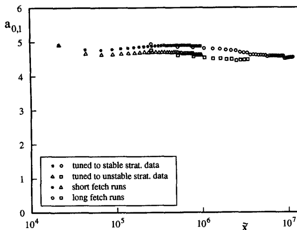
FIG. 4. Local estimates a_{0,l} [Eq. (42)] of a_0 in Eq. (32) as a function of the nondimensional fetch \tilde{x} for the four test cases: \alpha_r = 0.002 , a_2 = 2.0 for cases tuned to stable stratification data, and a_2 = 1.5 for cases tuned to unstable stratification data.
