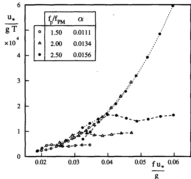
FIG. 1. Inverse nondimensional timescales \tilde{T}^{-1} = u_*/(gT) as a function of the nondimensional frequency f u_*/g for the input source term (dotted lines) and the nonlinear interactions (dashed lines) for several JONSWAP spectra with the directional distribution of Hasselmann et al. (1980). Results for 1.75 < f/f_p < 4 only.
