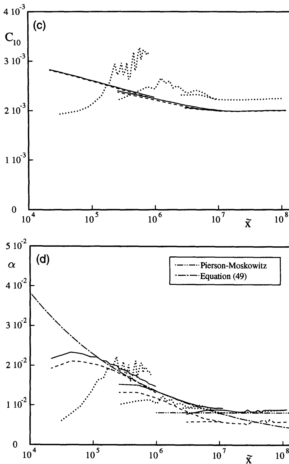
FIG. 7. (Continued) long-fetch case ( \Delta x = 2.5, 25 , and 250 km, respectively). The dark-shaded areas represent the envelope of the stable stratification data of Kahma and Calkoen (1992, 1994); the light represents all data.
