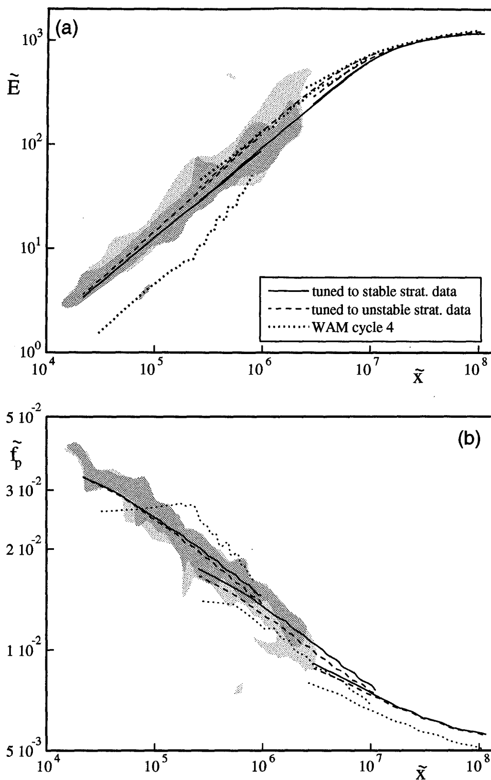
FIG. 7. Nondimensional energy \tilde{E} = Eg^2 u_*^{-4} (panel a), peak frequency \tilde{f}_p = f_p u_* g^{-1} (panel b), the drag coefficient at 10 m C_{10} = \sqrt{u_*}/u_{10} (panel c), and high-frequency energy level \alpha(f_c) (panel d) as a function of the nondimensional fetch \tilde{x} = xgu_*^{-1} for the conditions in which the model has been tuned and an additional
